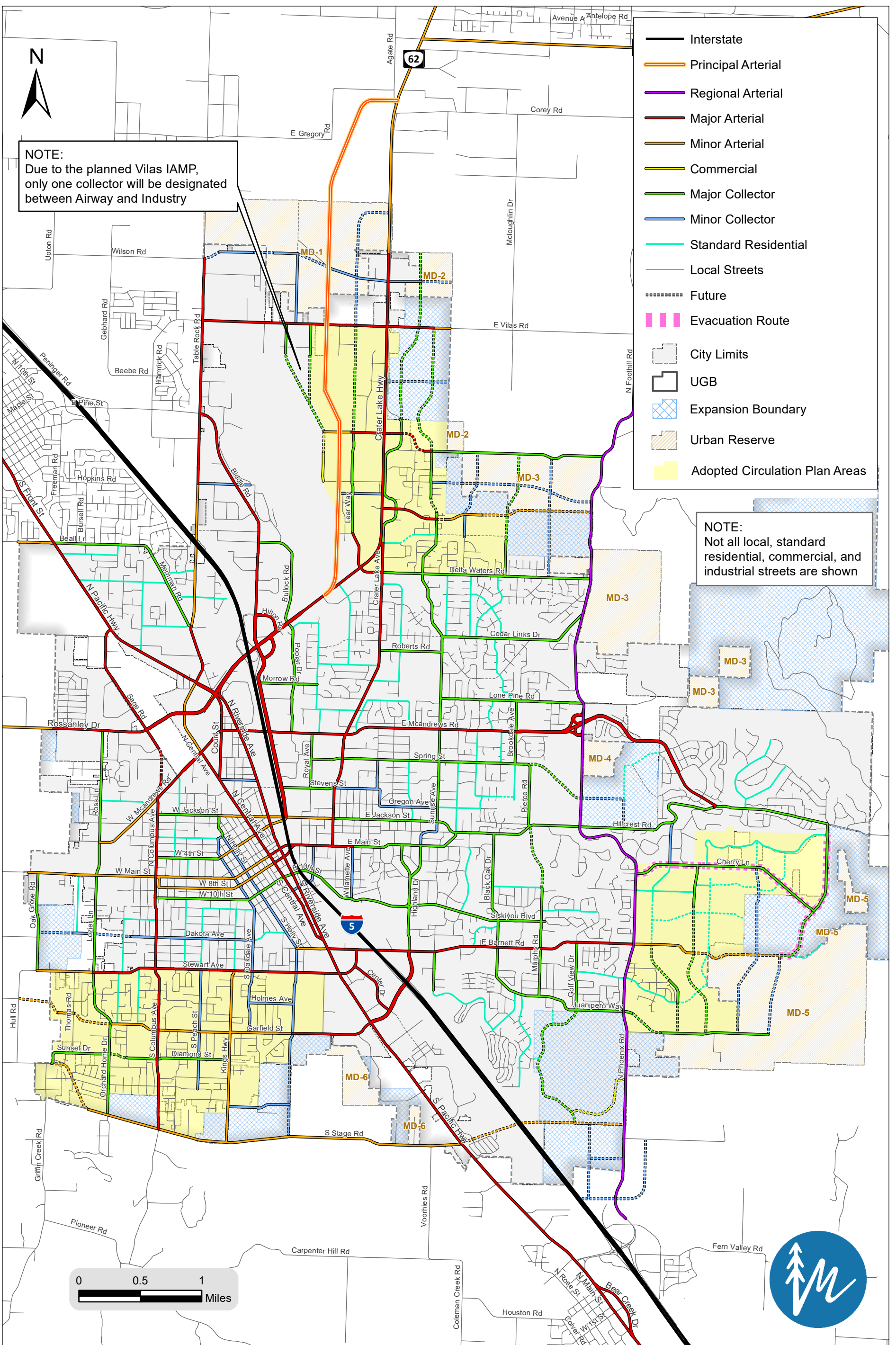
Roadway Functional Classification Map Medford, Oregon
